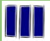
Multistructural
